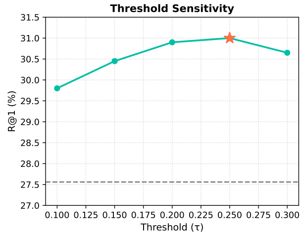
(b) Effect of confidence threshold \tau .
